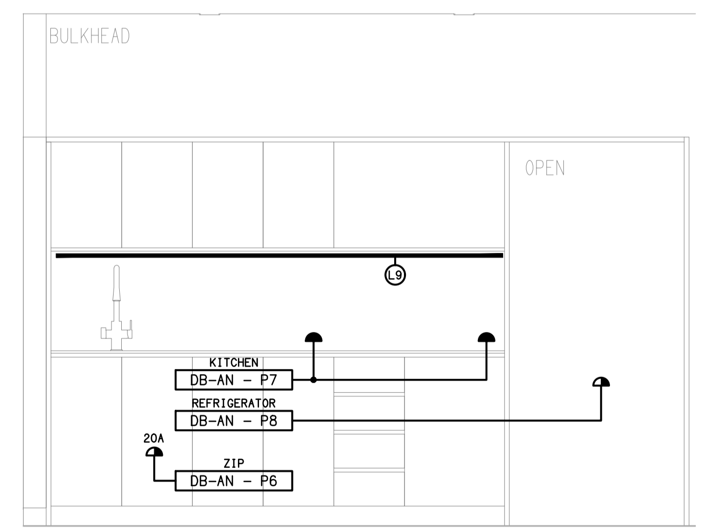
DETAIL A KITCHENETTE ELEVATION SCALE 1:20
